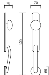
Art. 4140 Set America Set America
