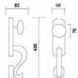
Art. 4102 Set America Set America
