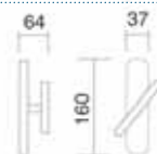
Art. 2792 Cremonese Window handle
