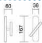
Art. 1802 Cremonese Window handle
