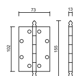
Art. 132 Cerniera piccola Small Hinge
