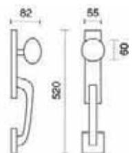
Art. 4125 Set America Set America
